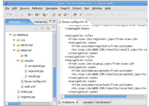
Figure 1: The view a JSF programmer has on source code of a web application
